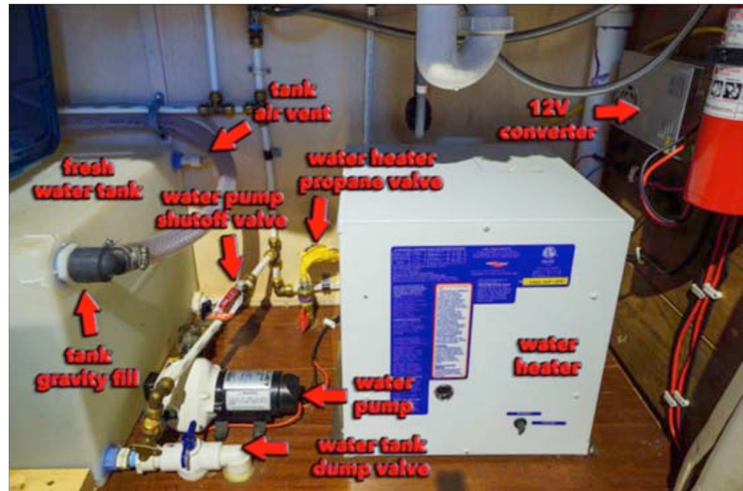
Jenna and Guillaume's water tank setup
